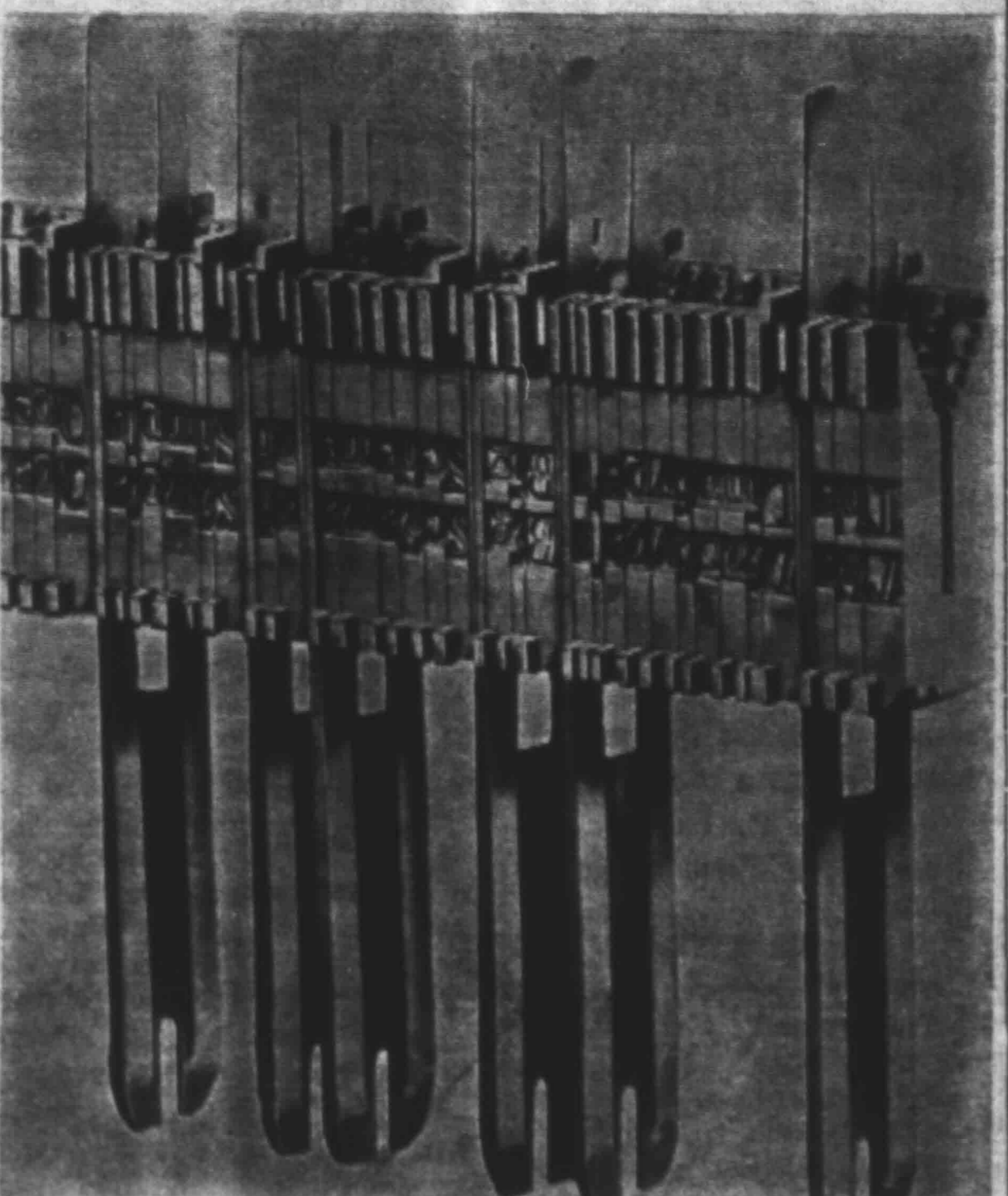
LINE OF MATRICES READY FOR CASTING includes wedge-shaped spacebands which were dropped between the words. Before casting, these are forced upward, filling the line out full width. On the top of the end matrix are visible the slide stop teeth which ride on the distributor bar. Differing combinations of these teeth on the matrices for different letters enable them to drop from the bar at proper places. Each matrix carries two type faces; those may be cast from either. The two are usually light face and bold face of the same style of type.
