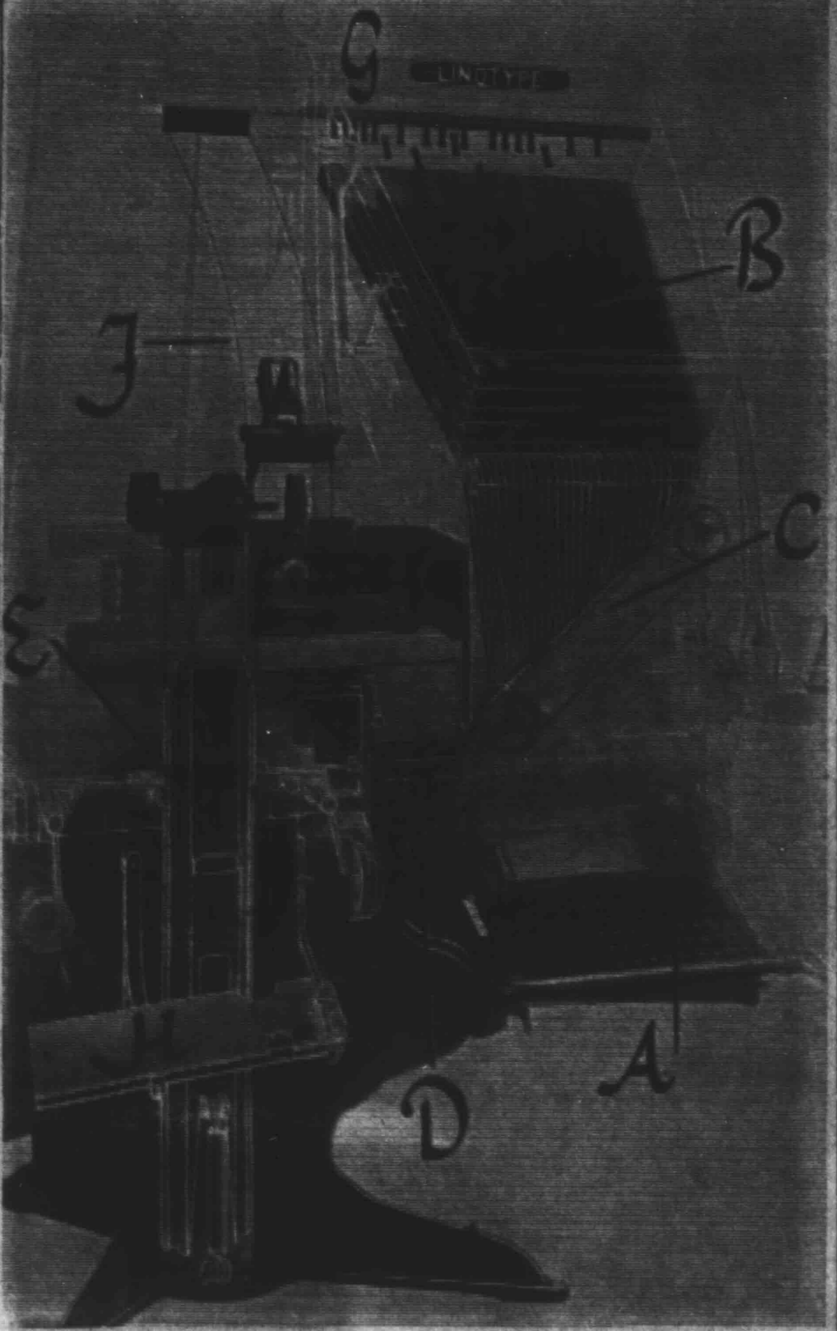
IN THE LINOTYPE, keyboard (A) releases brass molds, or matrices, of letters from storage channels in a magazine (B); they fall by gravity onto a bath (C) which assembles them where the operator can see them (D), and when the line is full, a solid slug is cast in mold (E) and drops into the galley (F). The matrices are raised (G) to the distributor bar (G) from which they drop back into proper channels.
